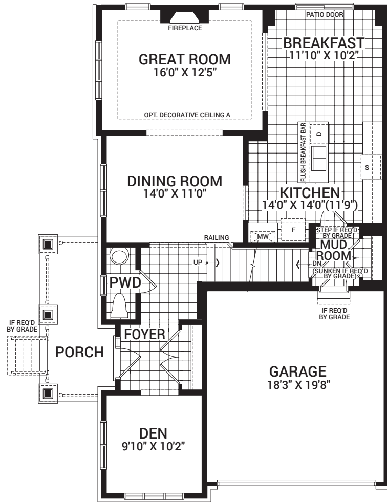
MAIN FLOOR
