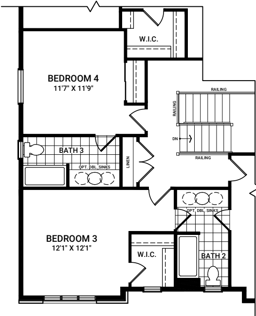
OPTIONAL SECOND FLOOR LAYOUT A
