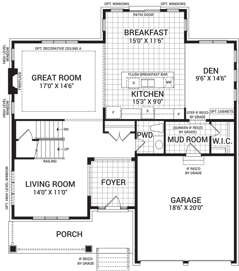
MAIN FLOOR
