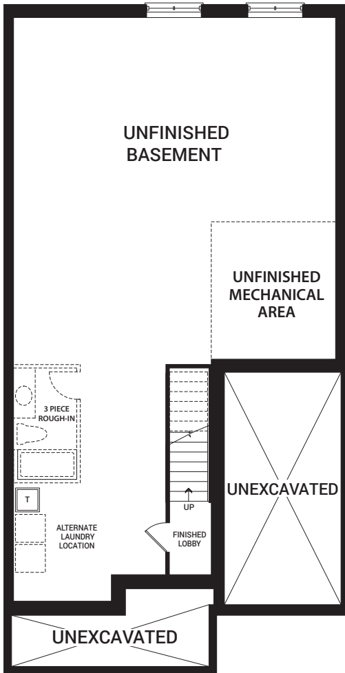
BASEMENT PLAN
