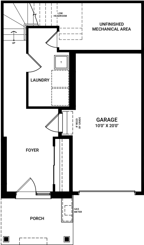
FIRST FLOOR ELEVATION A (SIMILAR FOR ELEVATION B)
