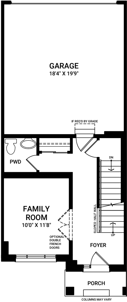
FIRST FLOOR ELEVATION A
