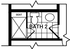
BATH 2 TUB TO 4 ft SHOWER PLUS BENCH
