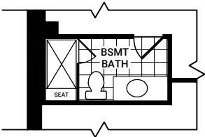
BASEMENT BATH TUB TO 4 ft SHOWER PLUS BENCH
