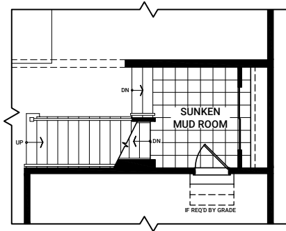
OPTIONAL OPEN BASEMENT STAIR
