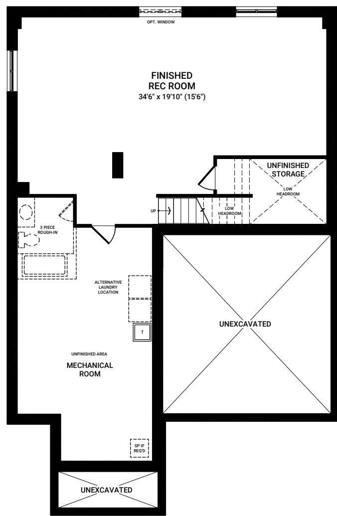
OPTIONAL FINISHED BASEMENT REC ROOM
