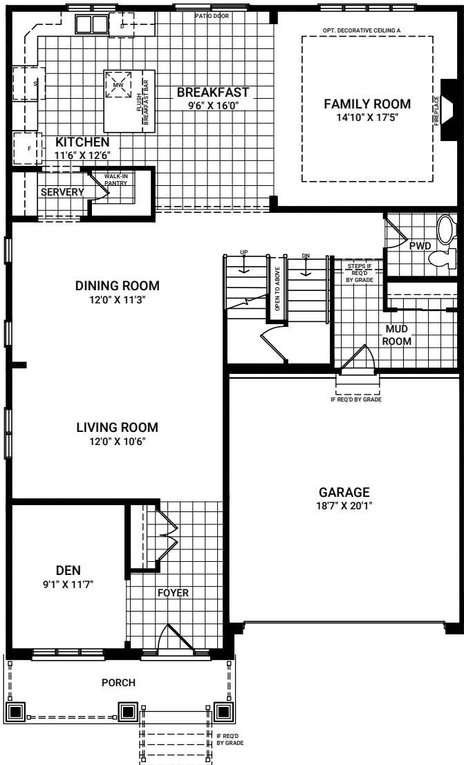
FIRST FLOOR ELEVATION C
