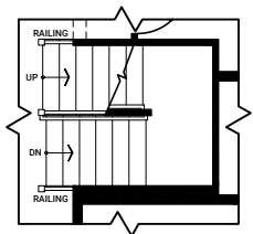
OPTIONAL OPEN BASEMENT STAIR
