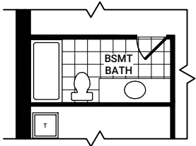
OPTIONAL BASEMENT 3 PIECE BATH
