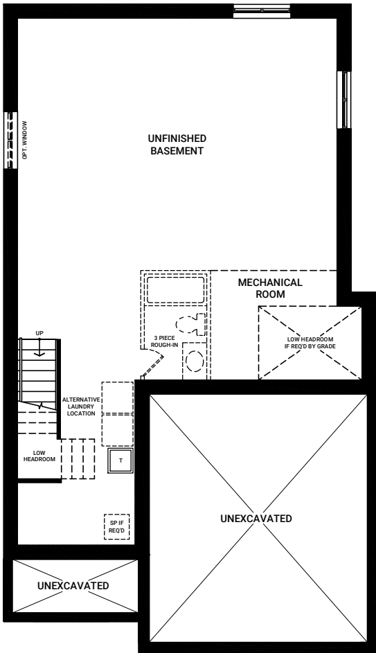
BASEMENT FLOOR ELEVATION A (SIMILAR FOR ELEVATIONS B, C & E)
