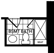
BASEMENT BATH TUB TO 4 ft SHOWER PLUS BENCH
