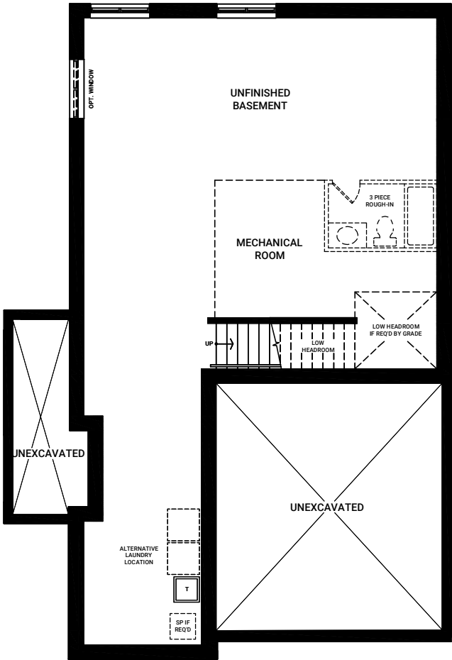
BASEMENT FLOOR ELEVATION D
