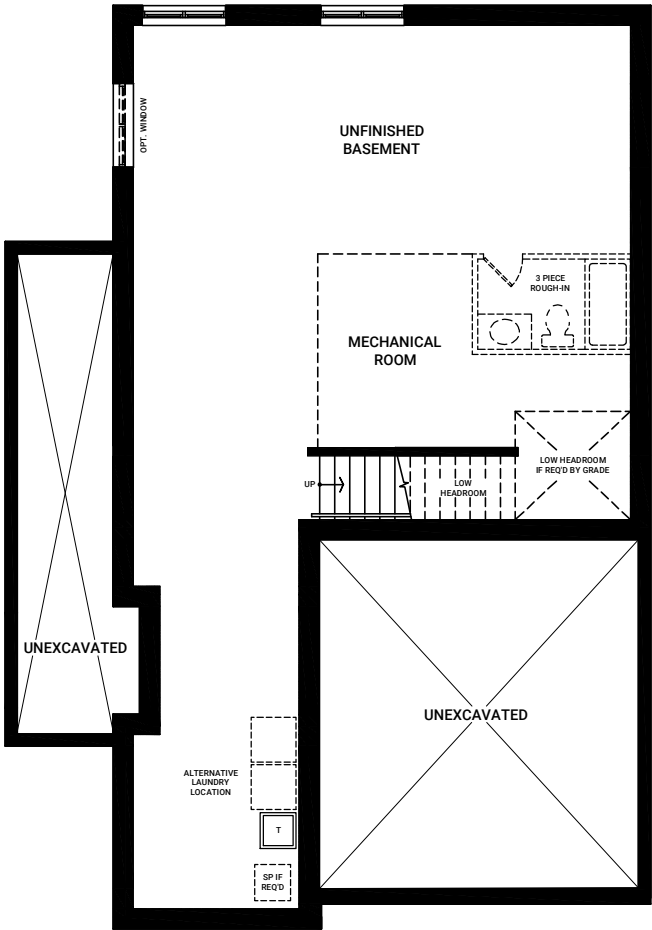
BASEMENT FLOOR ELEVATION B
