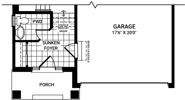
FIRST FLOOR ELEVATION E
