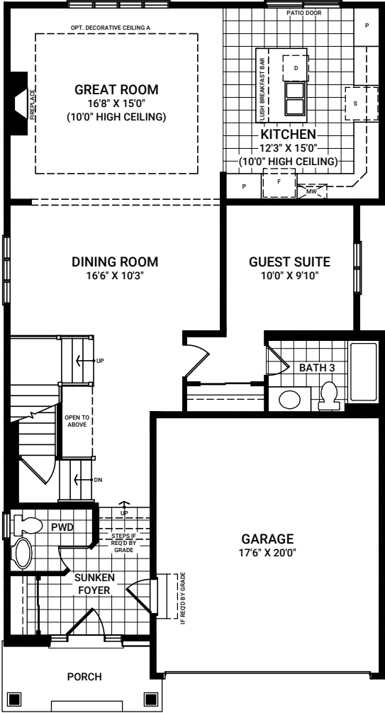
FIRST FLOOR ELEVATION A
