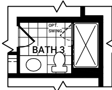
PRE-FAB BASE BATH 3 TUB TO 5 ft SHOWER
