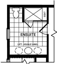
OPT. SECOND FLOOR LAYOUT A ENSUITE 4 ft SHOWER PLUS BENCH
