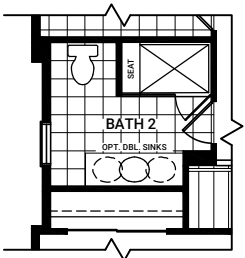
BATH 2 TUB TO 4 ft SHOWER PLUS BENCH
