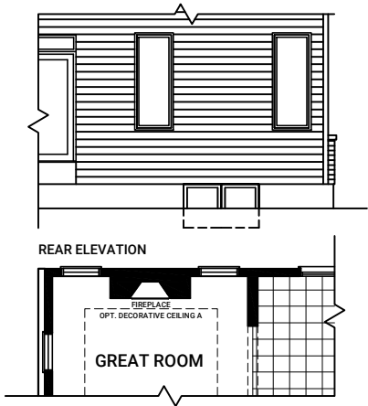
OPTIONAL GREAT ROOM WINDOWS AT REAR
