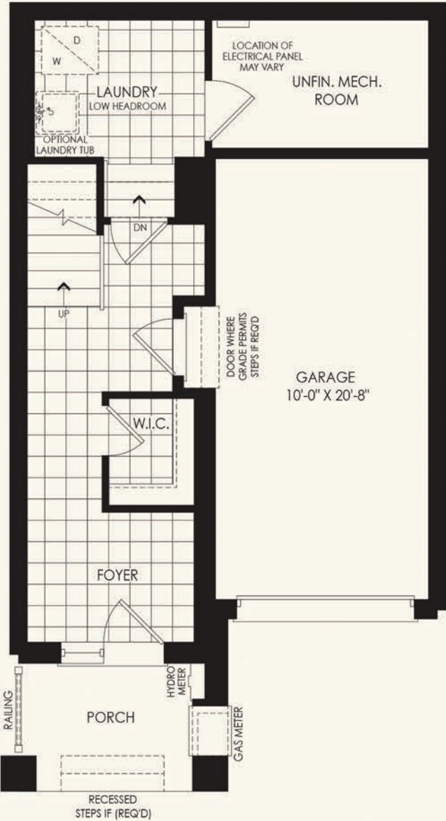
GROUND FLOOR PLAN ELEV. 'A'
