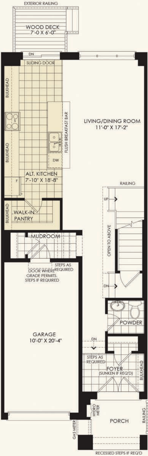
OPT. GROUND FLOOR PLAN W/ ALTERNATE KITCHEN ELEV 'A'
