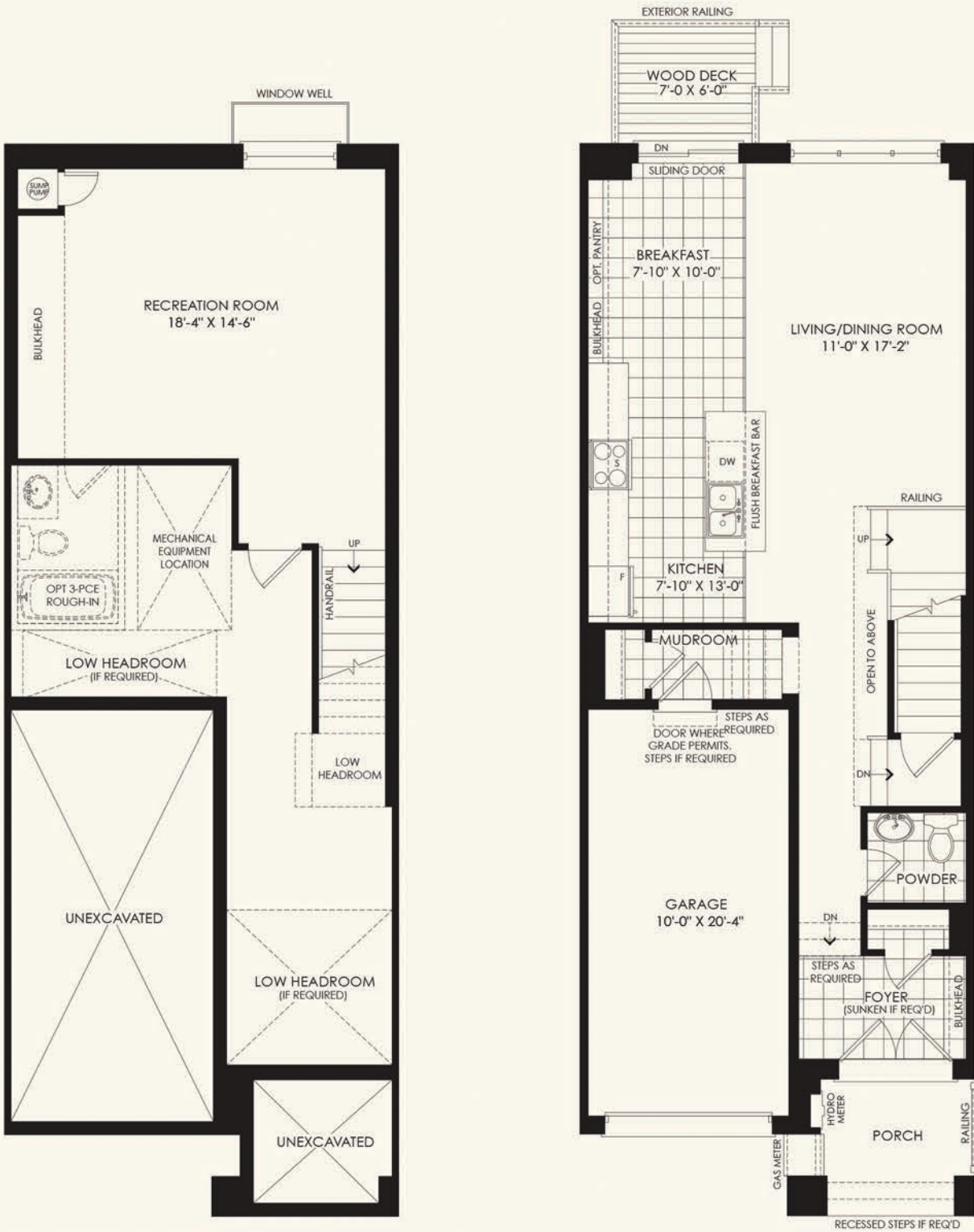
BASEMENT PLAN ELEV 'A' GROUND FLOOR PLAN ELEV 'A'
