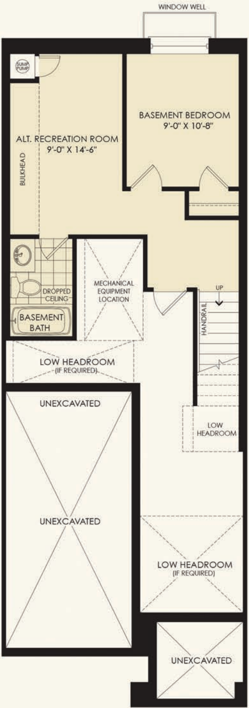
OPT. BASEMENT PLAN W/ ALT. REC ROOM, BASEMENT BEDROOM & BASEMENT BATHROOM ELEV. 'A' IF GRADE PERMITS
