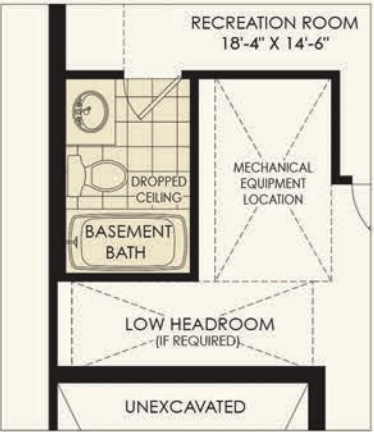
PARTIAL BASEMENT PLAN W/ 3 PC. BATHROOM ELEV. 'A'
