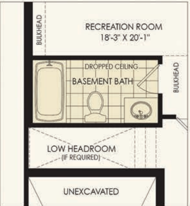
PARTIAL BASEMENT PLAN W/ 3 P.C. BATHROOM ELEV. 'A'
