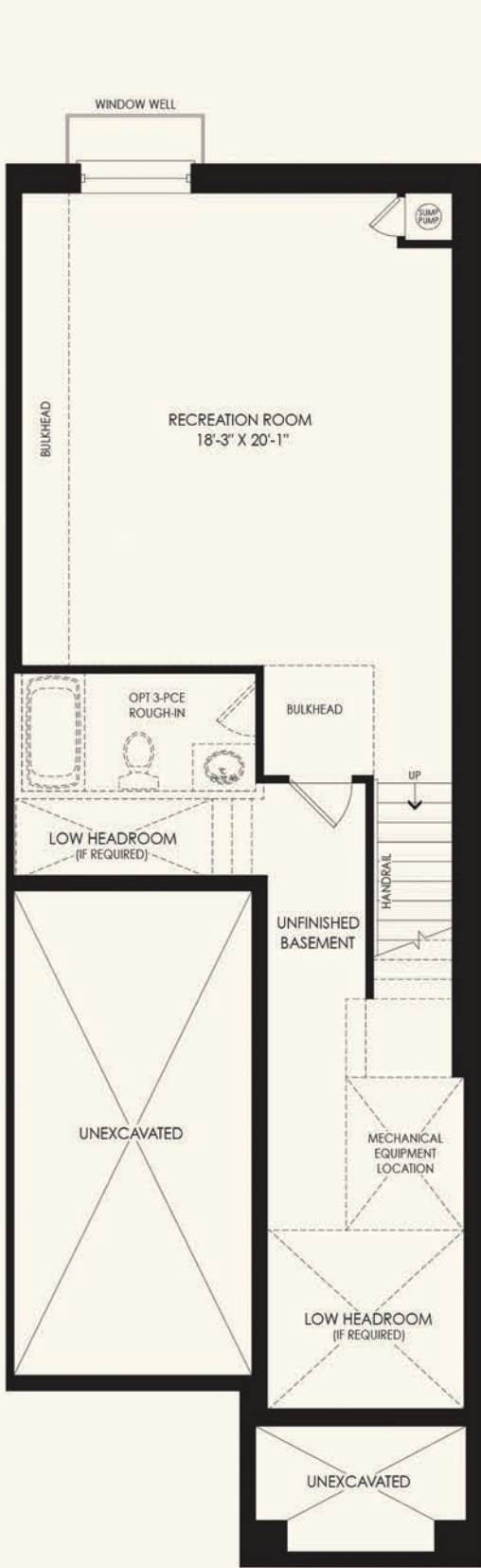
BASEMENT PLAN ELEV. 'A'
