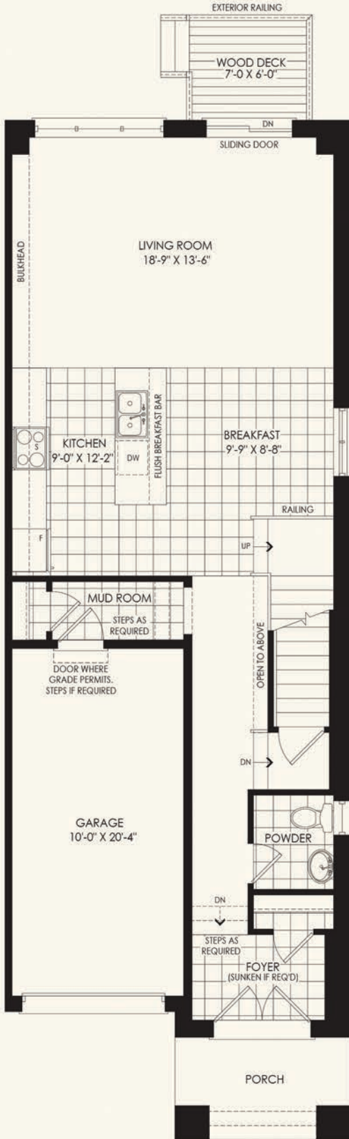
GROUND FLOOR PLAN ELEV. 'A'
