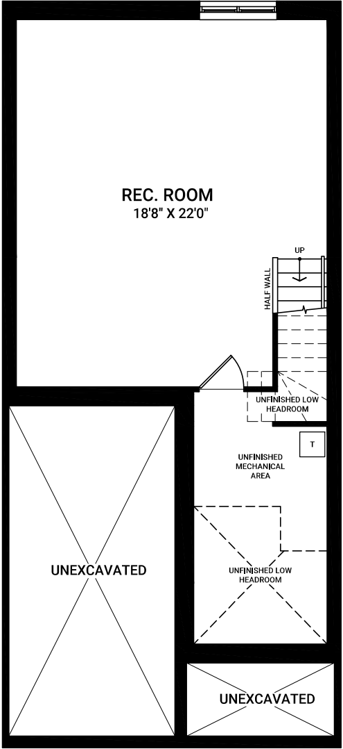
FINISHED BASEMENT ELEVATION A (SIMILAR FOR ELEVATIONS B & C)
