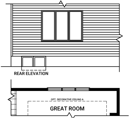
OPTIONAL LARGER WINDOW IN GREAT ROOM
