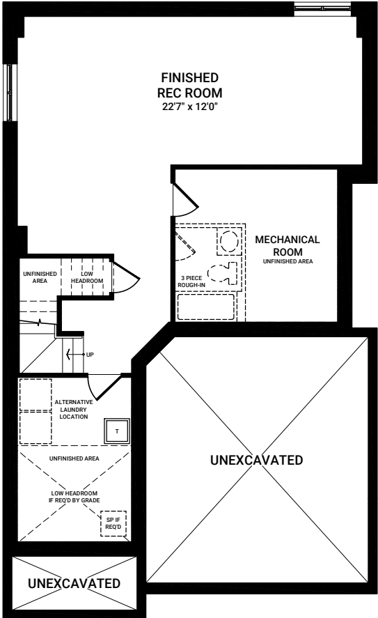
OPTIONAL FINISHED BASEMENT REC ROOM
