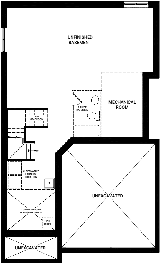
BASEMENT FLOOR ELEVATION A (SIMILAR FOR ELEVATIONS B & C)
