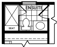
ENSUITE TUB TO 4 ft SHOWER PLUS BENCH
