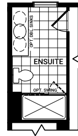
PRE-FAB BASE
