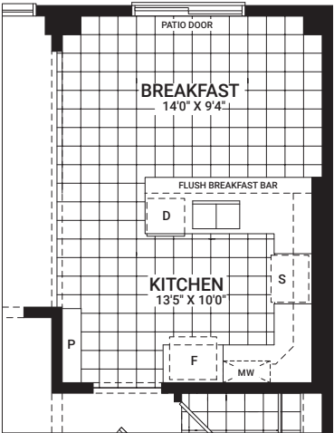
OPTIONAL KITCHEN LAYOUT A
