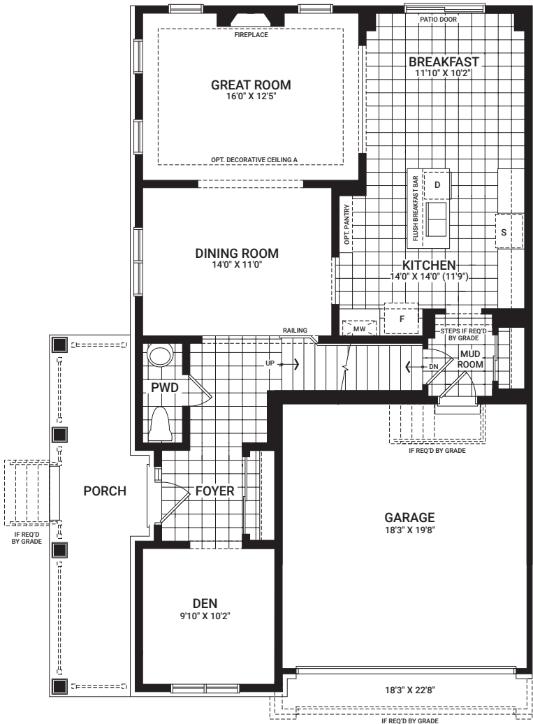
MAIN FLOOR
