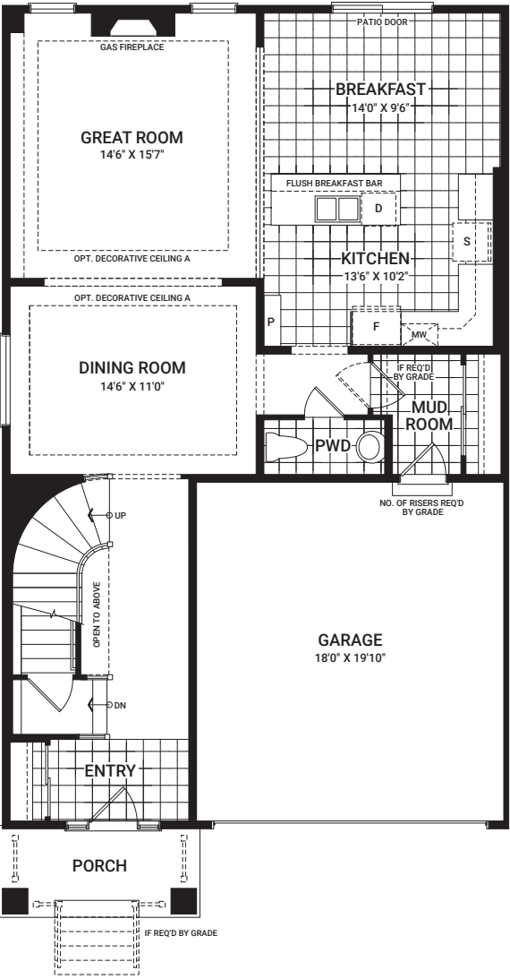
MAIN FLOOR
