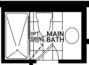
TUB TO 5 FT. SHOWER
