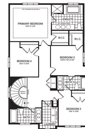
OPTIONAL SECOND FLOOR LAYOUT A
