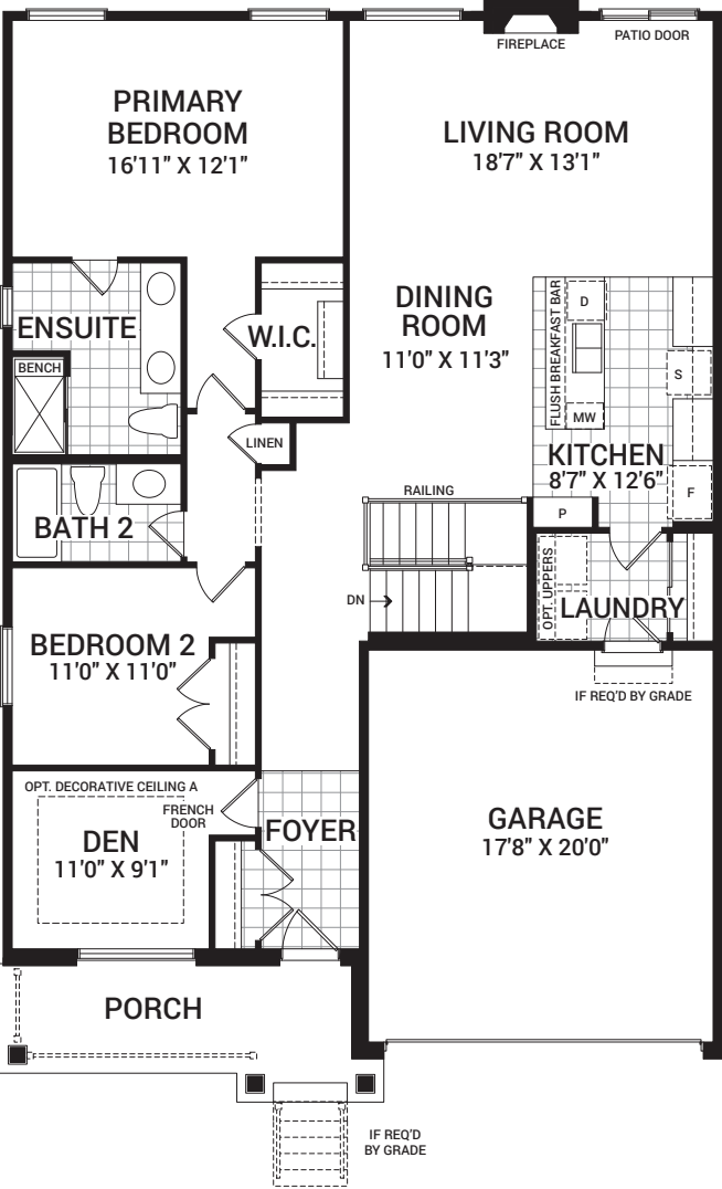
MAIN FLOOR
