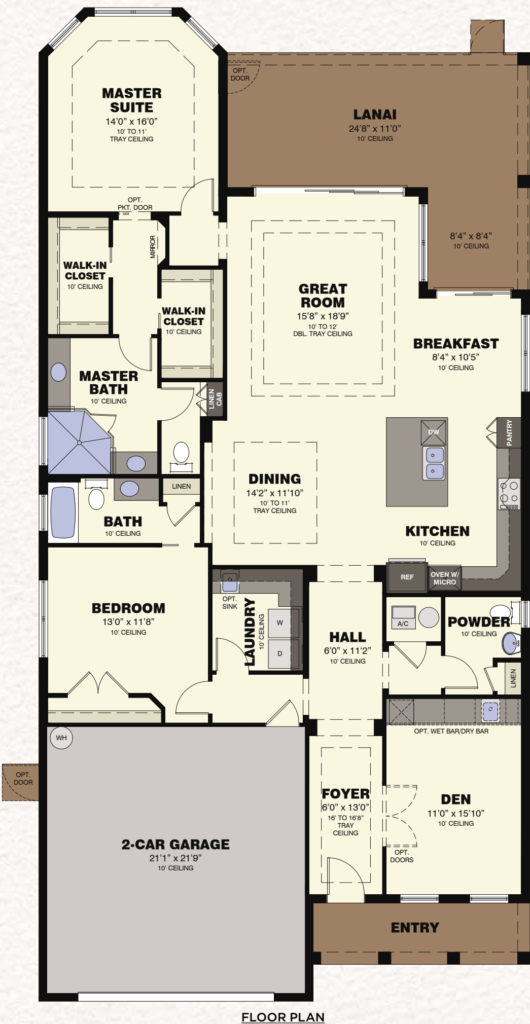
FLOOR PLAN
