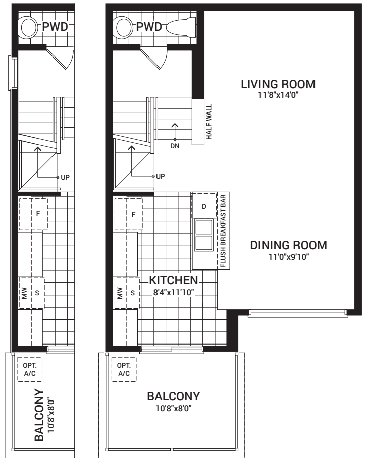
END UNIT SECOND FLOOR PLAN
