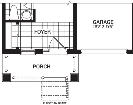
MAIN FLOOR PLAN B
