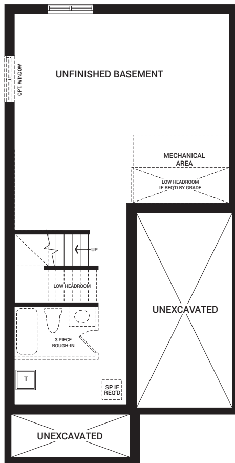
BASEMENT FLOOR PLAN A (SIMILAR FOR PLAN B, C & D)
