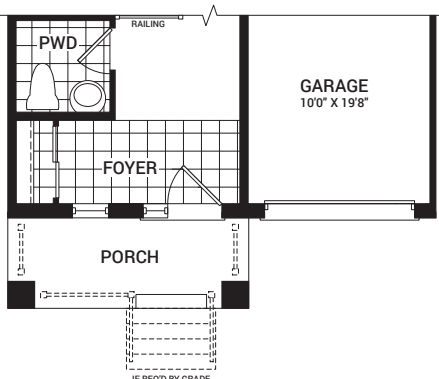
MAIN FLOOR PLAN D
