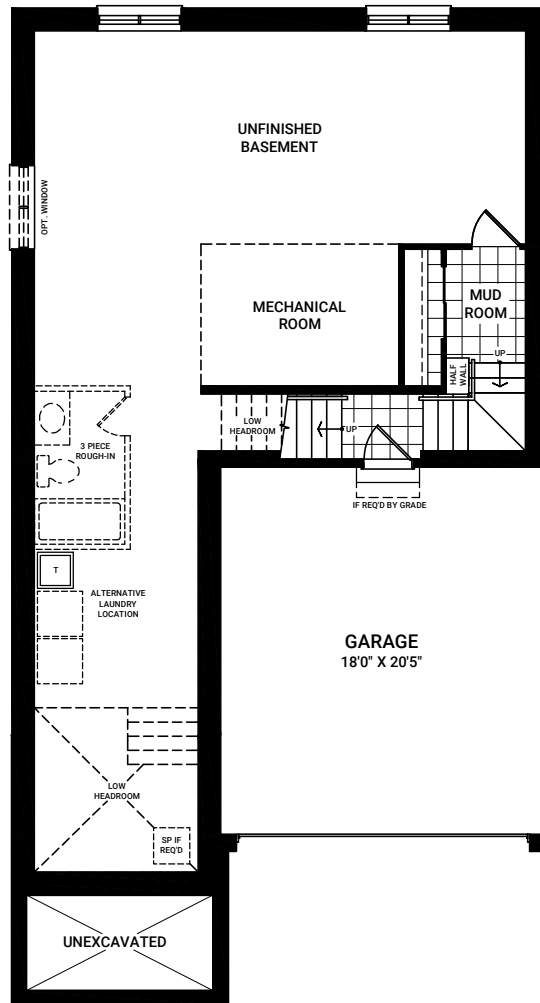
BASEMENT FLOOR ELEVATION A (SIMILAR FOR ELEVATION C)
