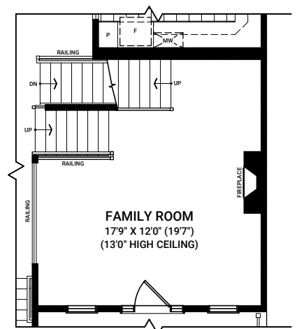
(RELOCATE FIREPLACE FROM GREAT ROOM) ADD FIREPLACE TO FAMILY ROOM OR RELOCATE FIREPLACE TO FAMILY ROOM
