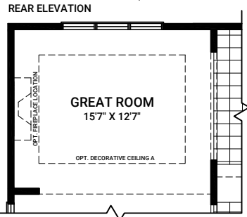
(RELOCATE FIREPLACE) OPTIONAL LARGER WINDOW IN GREAT ROOM
