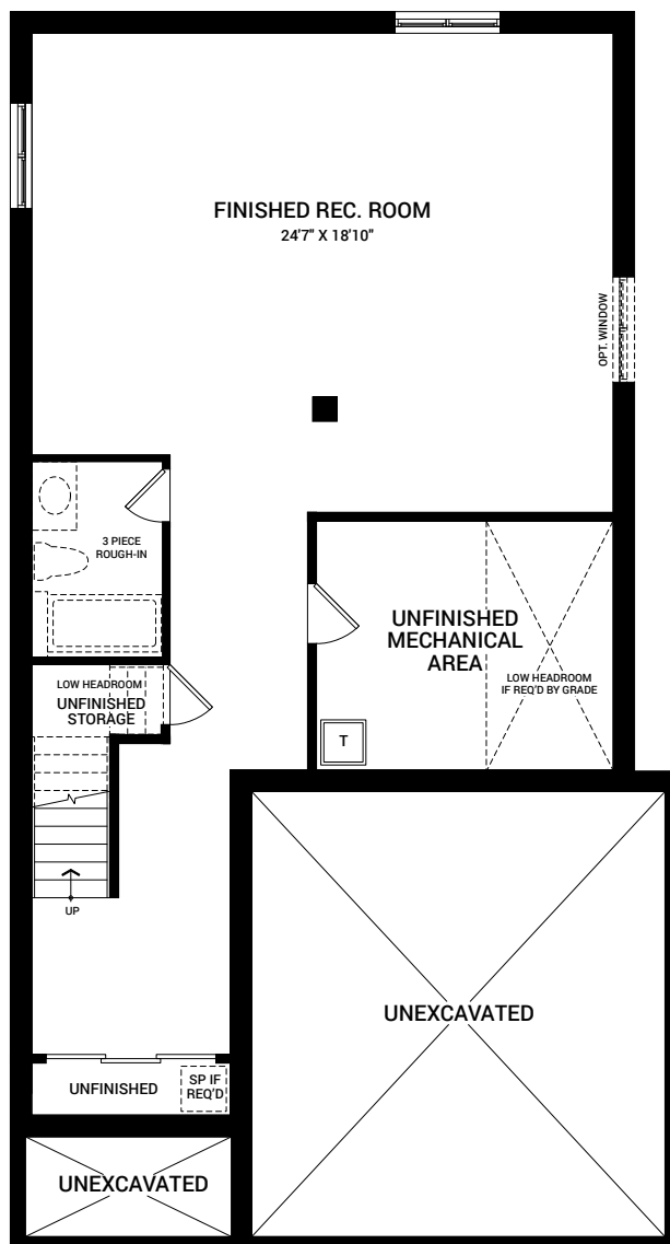
OPTIONAL FINISHED BASEMENT REC. ROOM
