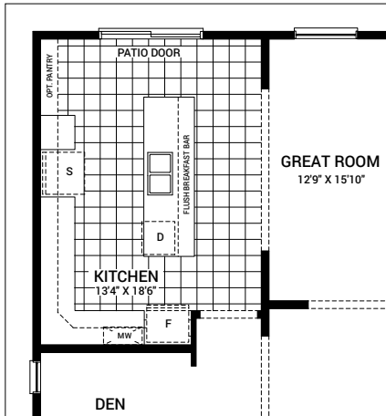
OPTIONAL KITCHEN LAYOUT A
