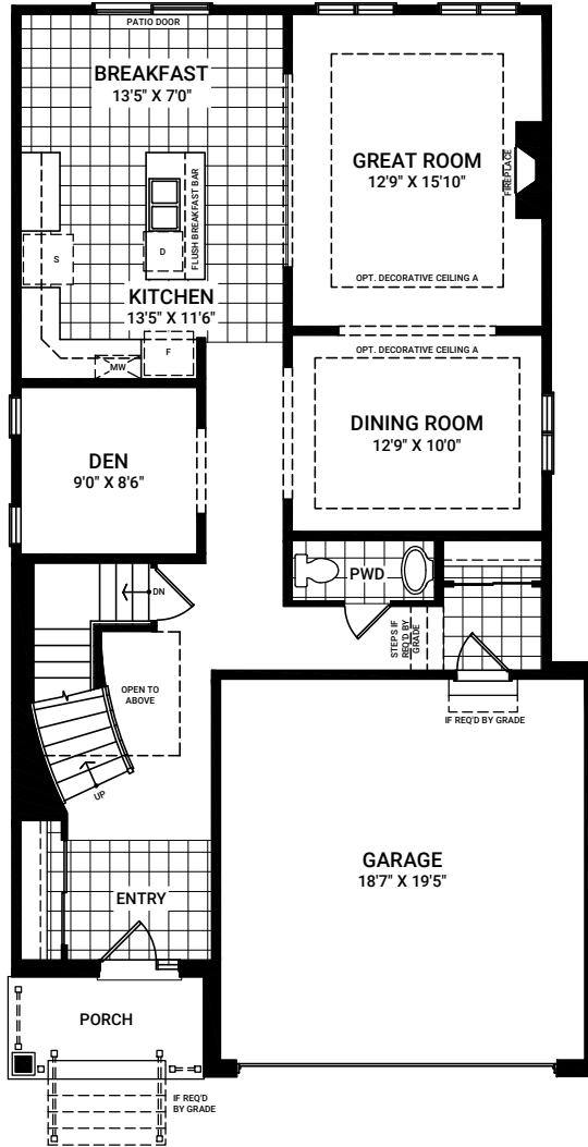
FIRST FLOOR ELEVATION A
