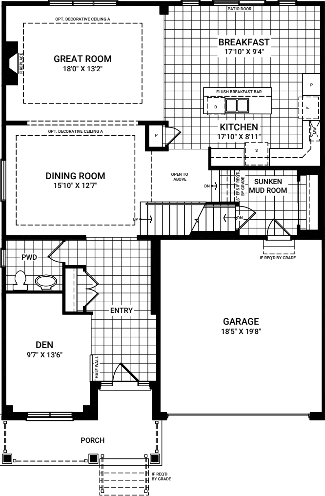
FIRST FLOOR ELEVATION A
