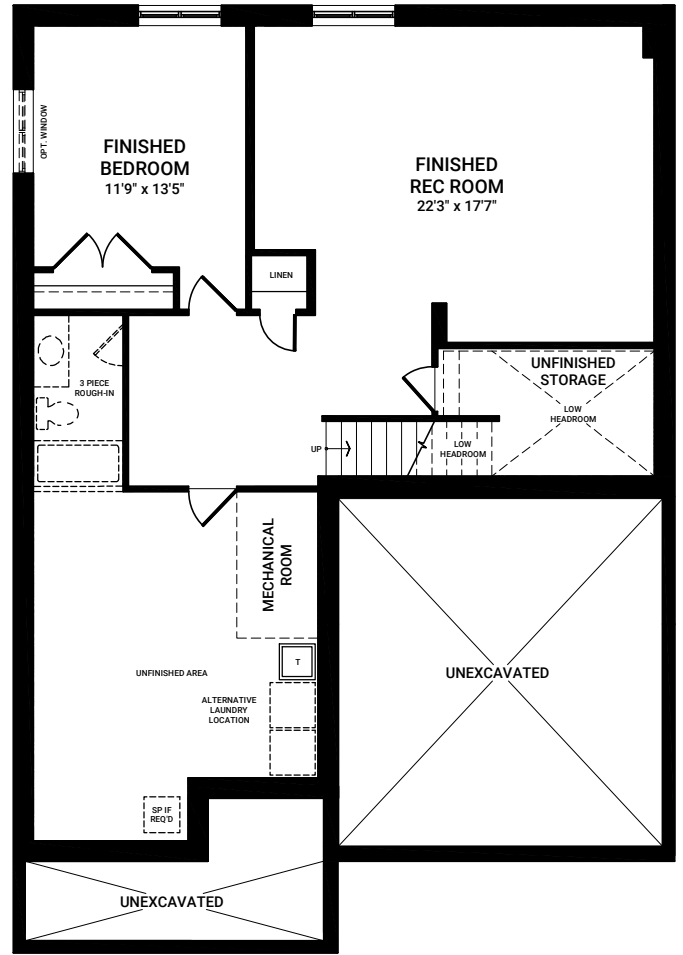
OPTIONAL FINISHED BASEMENT REC ROOM WITH BEDROOM
