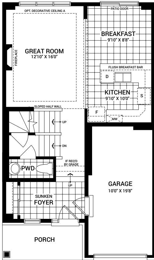
MAIN FLOOR PLAN A
