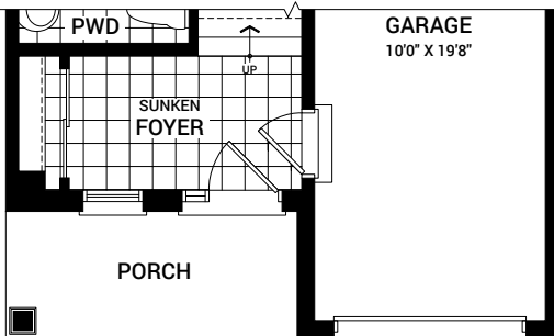
MAIN FLOOR PLAN B
