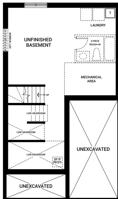
BASEMENT FLOOR PLAN A (SIMILAR FOR PLAN B AND C)
