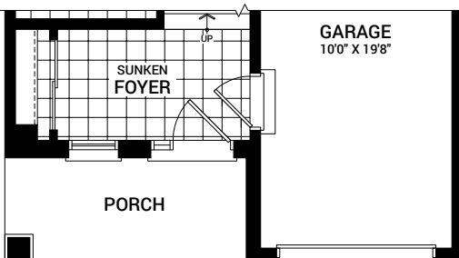
MAIN FLOOR PLAN C
