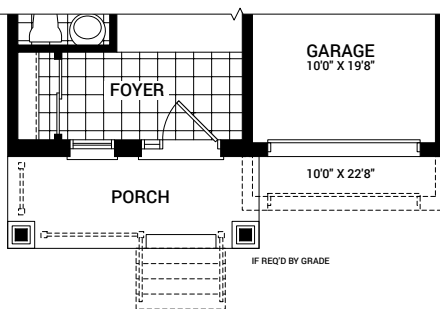
MAIN FLOOR PLAN C
