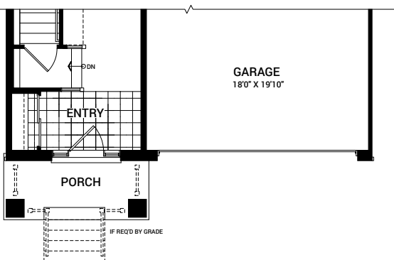
MAIN FLOOR PLAN D
