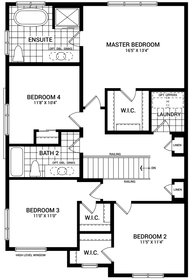
SECOND FLOOR PLAN D
