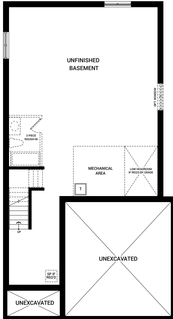
BASEMENT FLOOR PLAN A (SIMILAR FOR PLAN B, C & D)
