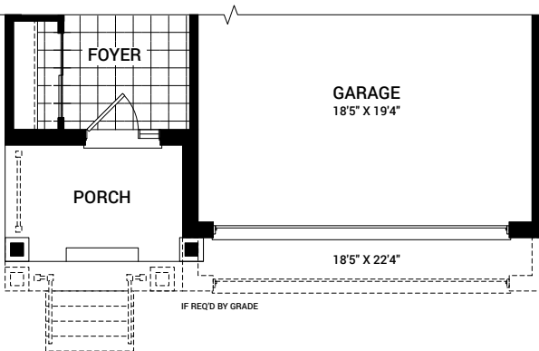
MAIN FLOOR PLAN B & C
