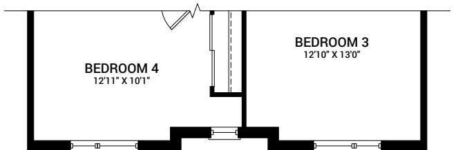
SECOND FLOOR PLAN D
