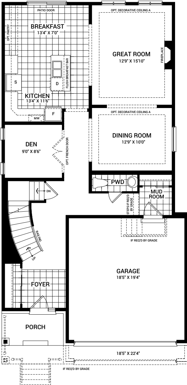
MAIN FLOOR PLAN A
