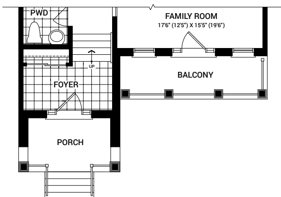
MAIN FLOOR PLAN C
