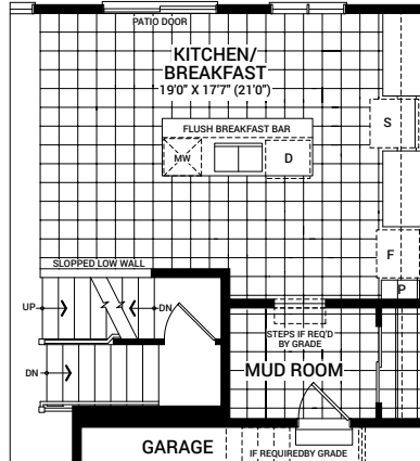
OPTIONAL KITCHEN LAYOUT FLEX PLAN OPTION
