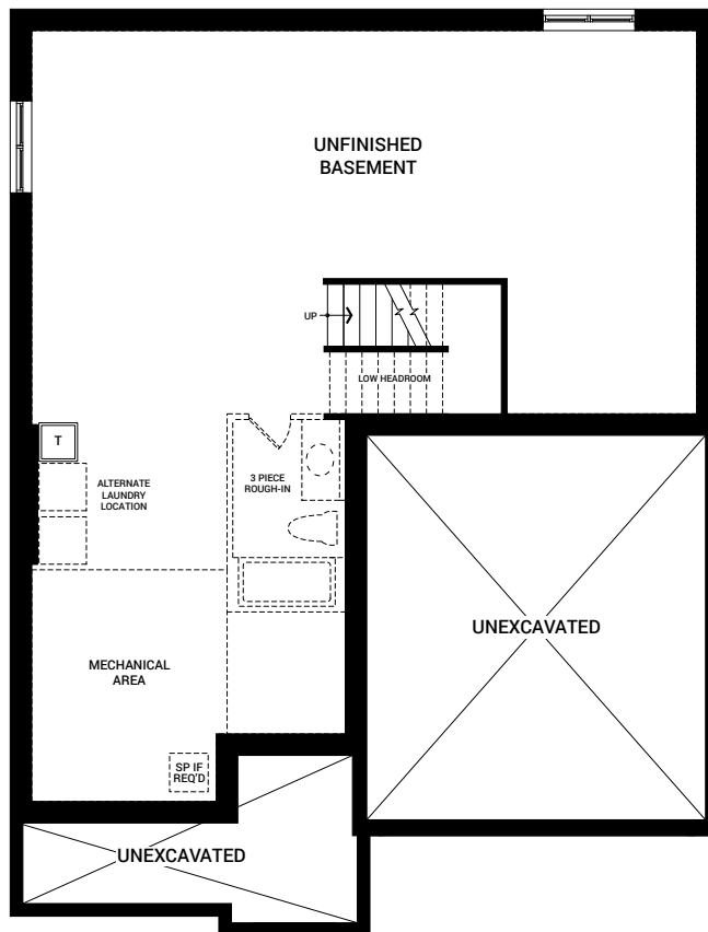
BASEMENT FLOOR PLAN A (SIMILAR FOR PLAN B & C)
