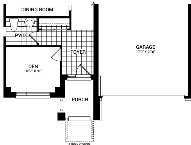
MAIN FLOOR PLAN C
