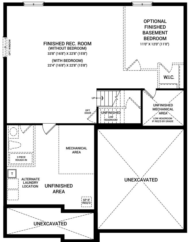
OPTIONAL FINISHED BASEMENT REC. ROOM W/ OPTIONAL BEDROOM (SIMILAR FOR PLAN C & D)
