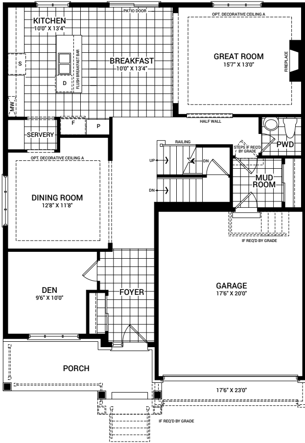
MAIN FLOOR PLAN A
