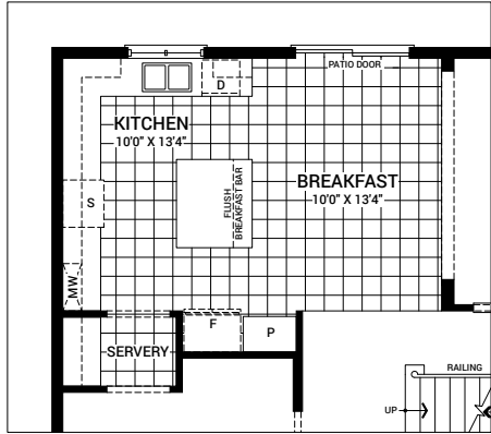
OPTIONAL KITCHEN LAYOUT A
