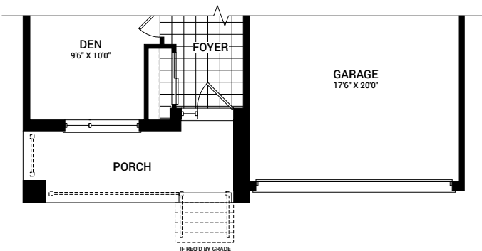
MAIN FLOOR PLAN D
