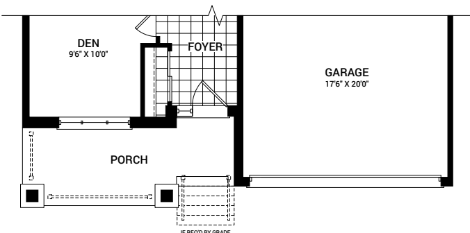
MAIN FLOOR PLAN C
