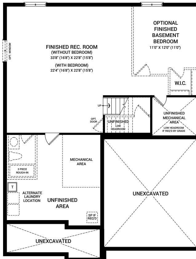
OPTIONAL FINISHED BASEMENT REC. ROOM W/ OPTIONAL BEDROOM (SIMILAR FOR PLAN C & D)
