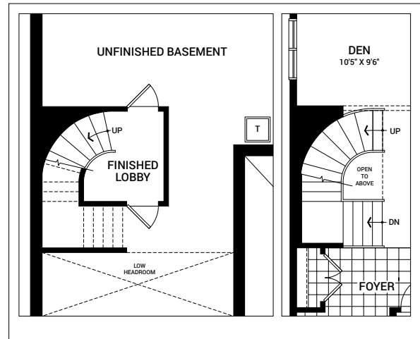
OPEN CIRCULAR FINISHED BASEMENT STAIRCASE WITH FINISHED LOBBY
