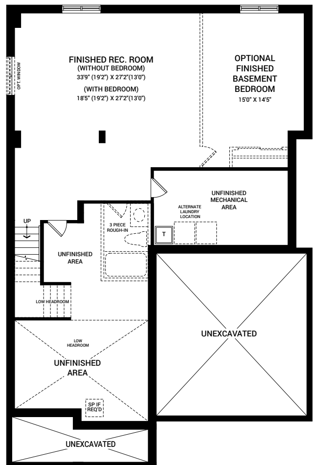
OPTIONAL FINISHED BASEMENT REC. ROOM W/ OPTIONAL BEDROOM (SIMILAR FOR PLAN B & D)
