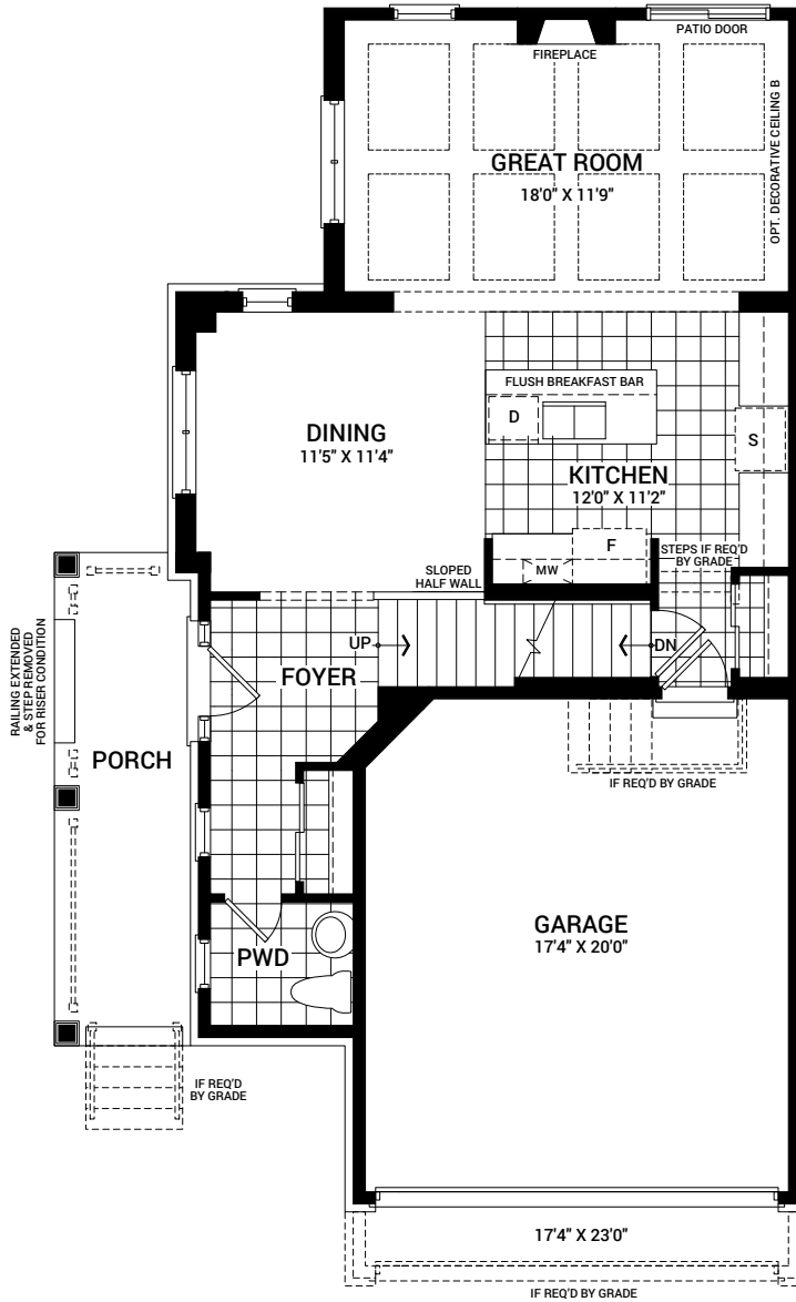
MAIN FLOOR PLAN A
