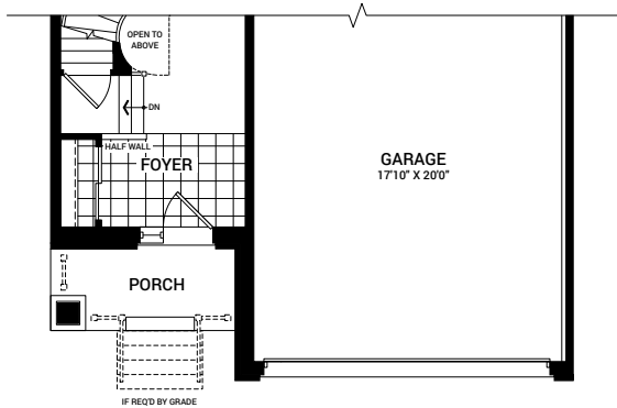
MAIN FLOOR PLAN B
