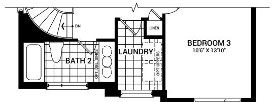
SECOND FLOOR PLAN D
