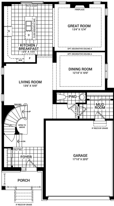
MAIN FLOOR PLAN A
