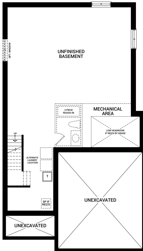
BASEMENT FLOOR PLAN A (SIMILAR FOR PLAN B, C & D)
