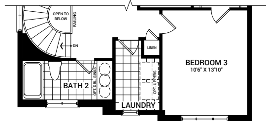
SECOND FLOOR PLAN B
