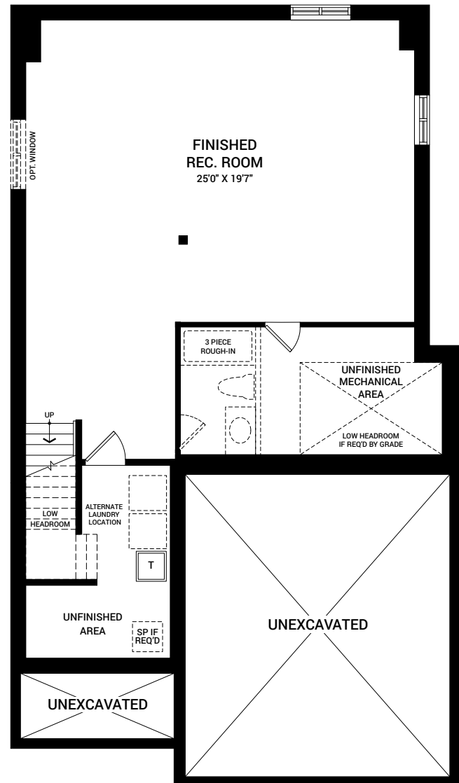
OPTIONAL FINISHED BASEMENT REC. ROOM
