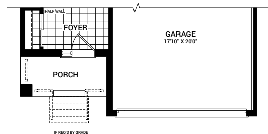
MAIN FLOOR PLAN D
