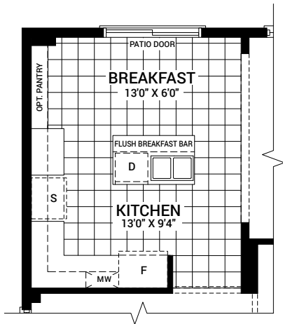
OPTIONAL KITCHEN LAYOUT A
