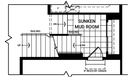
OPTIONAL OPEN BASEMENT STAIR
