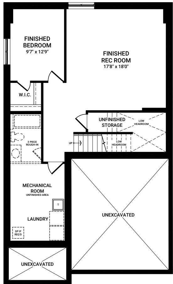
OPTIONAL FINISHED BASEMENT REC ROOM WITH BEDROOM
