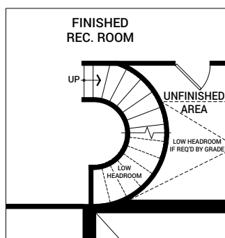
OPTIONAL CIRCULAR BASEMENT STAIR (UNFINISHED)
