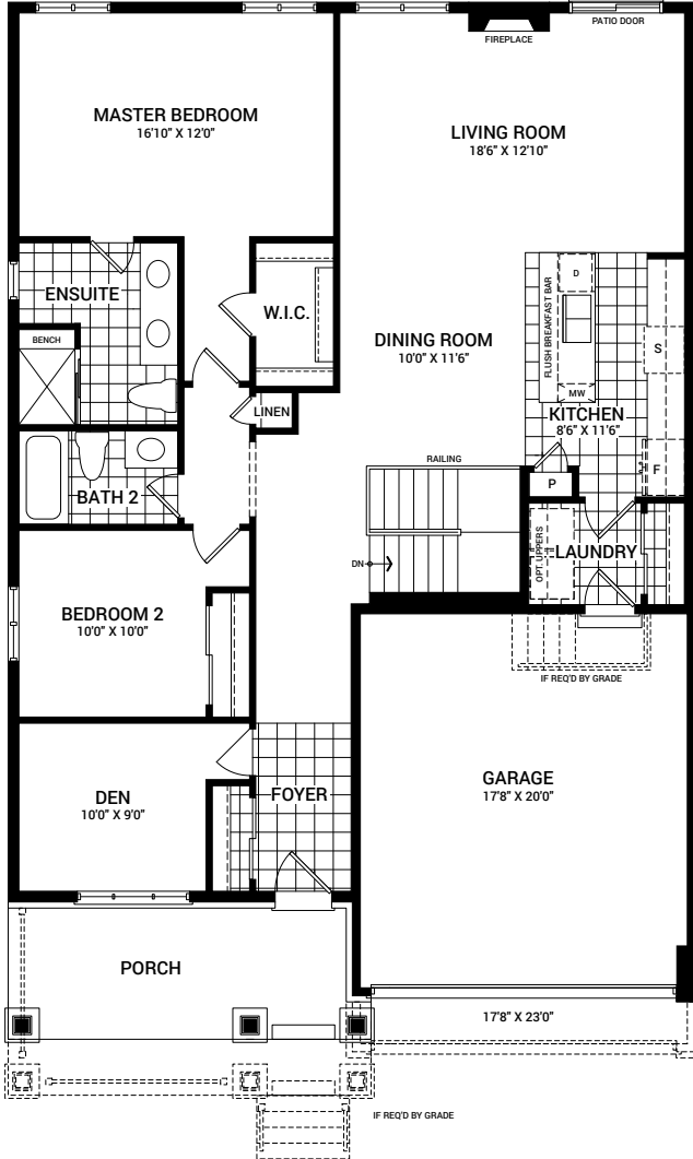
MAIN FLOOR PLAN A
