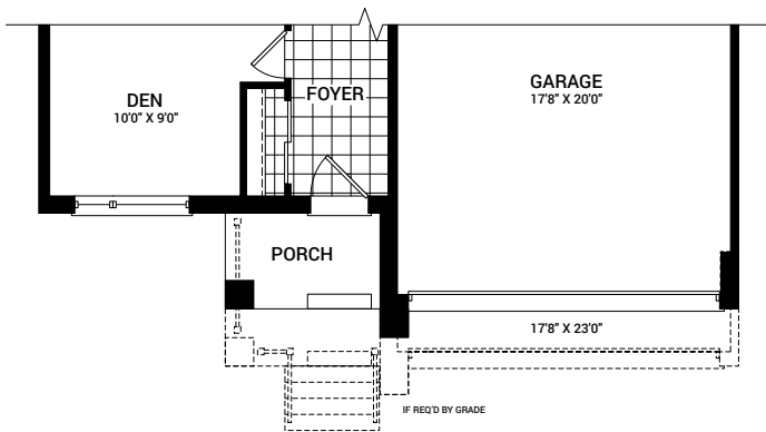
MAIN FLOOR PLAN B
