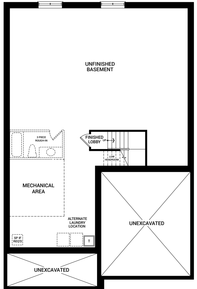
BASEMENT FLOOR PLAN A (SIMILAR FOR PLAN B)
