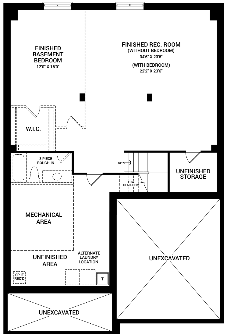
OPTIONAL FINISHED BASEMENT LAYOUT W/ OPTIONAL BEDROOM (SIMILAR FOR PLAN B)
