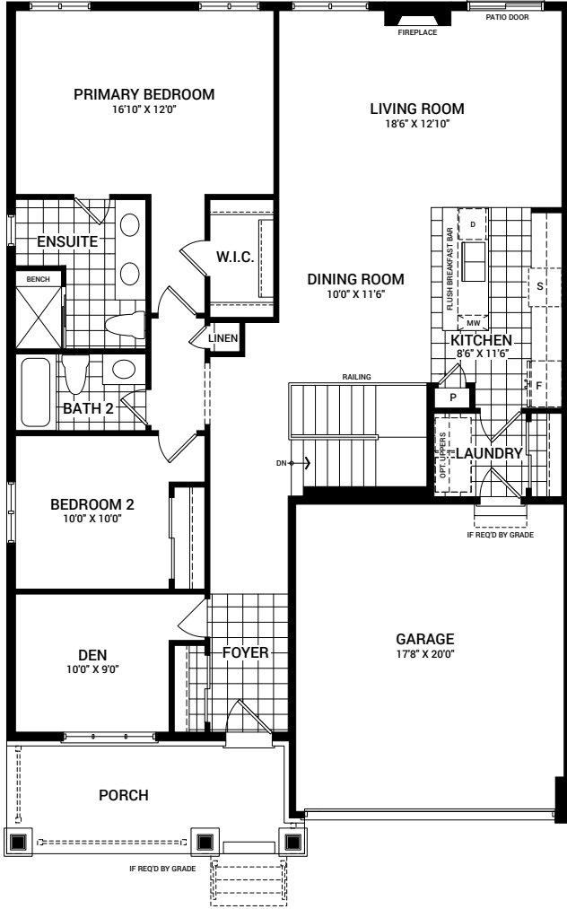
MAIN FLOOR PLAN A
