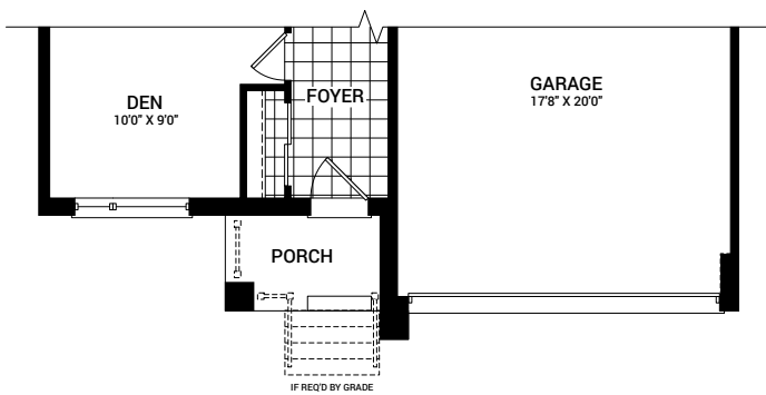
MAIN FLOOR PLAN B
