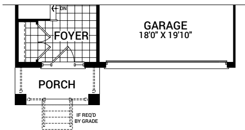
MAIN FLOOR PLAN C
